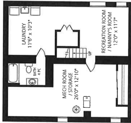
LOWER LEVEL 945 SQUARE FEET
