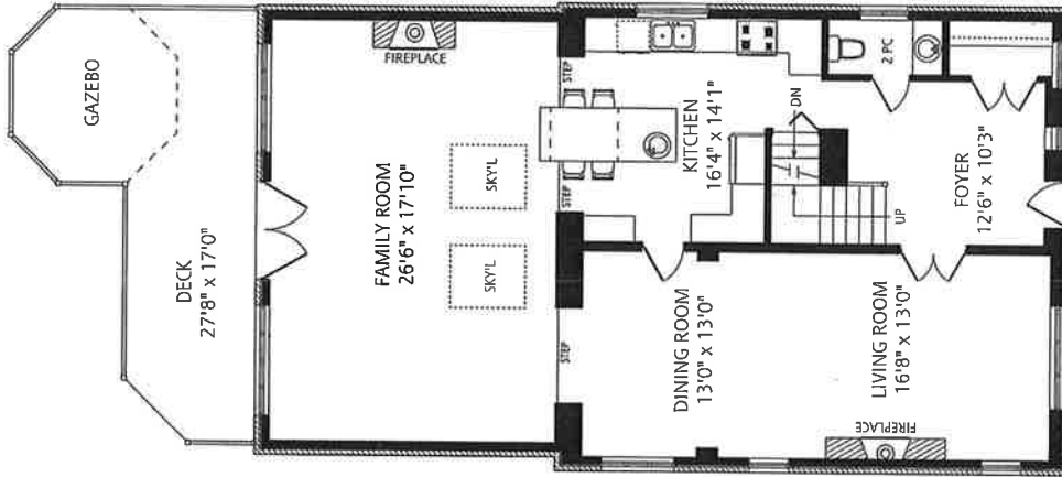
MAIN FLOOR 1,490 SQUARE FEET ALL MEASUREMENTS SHOULD BE CONSIDERED APPROXIMATE 1/8" = 1' SCALE
